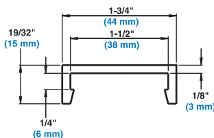
BARBED CLIP-ON (B6XX23IXXWMV-00)
