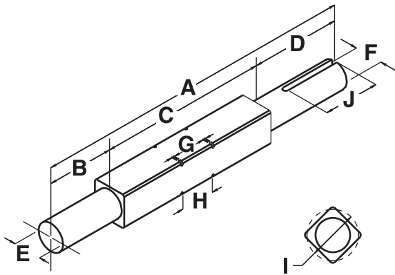
Fig. 2-16 Shaft dimensions
