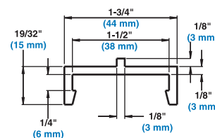
BARBED CLIP-ON WITH LEG (B6XX24IXXWMV-00)
