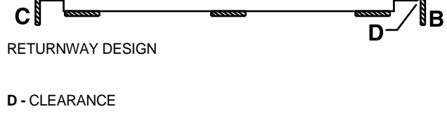
Fig. 2-5 HOLD DOWN RAILS AND WEARSTRIPS FOR SERIES 2400 FLAT-TURNS - HIGH DECK AND RAISED RIB BELTS
