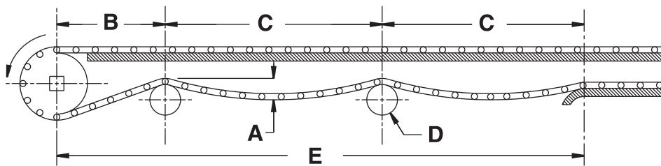
Fig. 3-12 Medium to long conveyors (6' [1.8 m] and longer)
