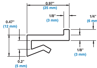
CLIP-ON WITH LEG (B6XX26IXXWMV-00)
