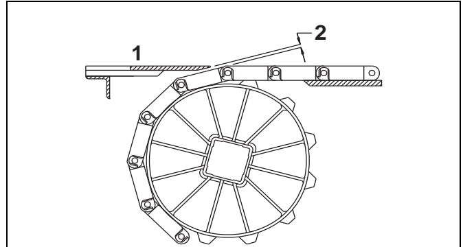
1 - Top surface of dead plate 2 - Dead plate gap
