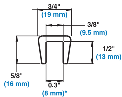
STANDARD BAR SNAP-ON (B6XX28IXXWMV-00) *min. (toe in)
