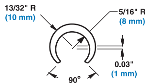
FULL ROUND SNAP-ON (B6XX29IXXWMV-00)
