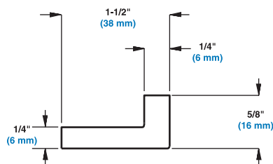
STANDARD ANGLE WEARSTRIP (B6XX21IXXWMV-00)
