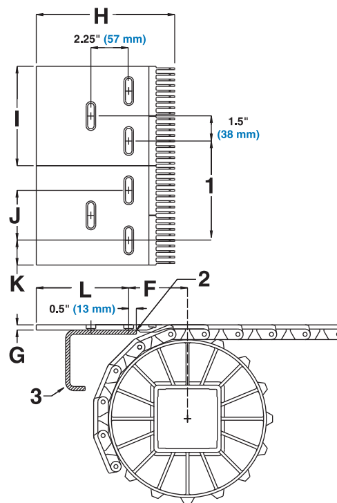
TWO-MATERIAL FINGER TRANSFER PLATES
