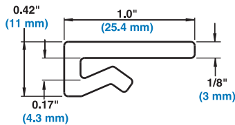
CLIP-ON (B6XX25IXXWMV-00)
