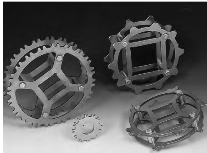
Fig. 2-28 Abrasion resistant (all steel) sprockets
