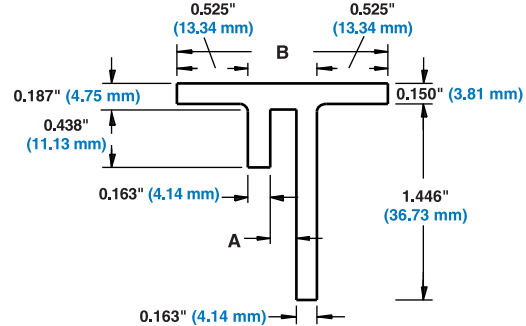
RADIUS BELT WEARSTRIP, CENTER RAIL HOLD DOWN WEARSTRIP
