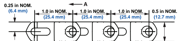
A -Preferred direction for flat turning applications
