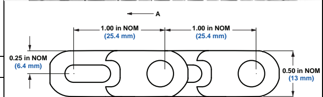
A - Preferred direction for flat turning applications
