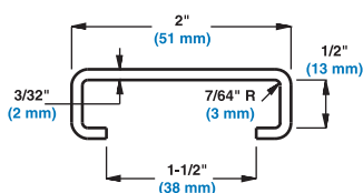
GUIDE RAIL SNAP-ON (B6XX27IXXWMV-00)
